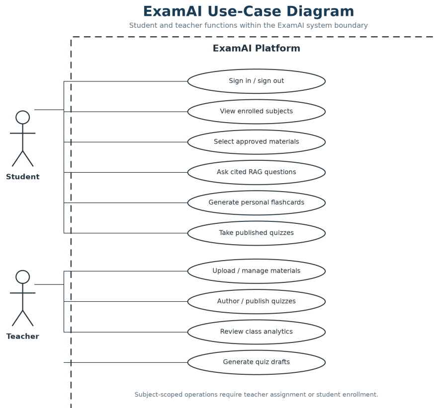
Figure 7.3: Use-case diagram
